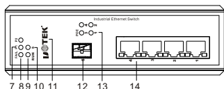
UT-6405GM-4GT1GSC-POE
